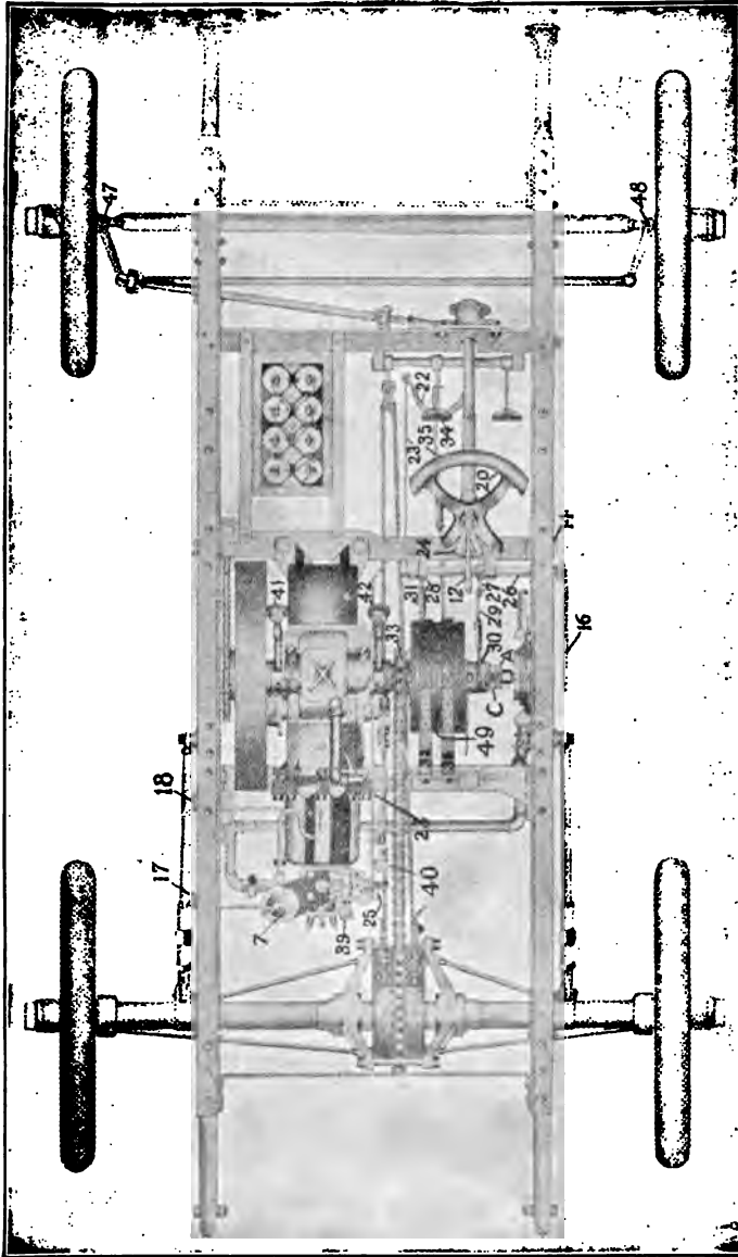
FIG. 248.—Plan View of the Cadillac Single-cylinder Runabout. The parts are: Carburetter (7); throttle lever (12); starting crank shaft (11); speed control lever (16); carburetter primer (17); windshield (18); drain valve (19); steering wheel (20); throttle connection (21); flywheel (22) shown at (22); throttle or valve control rod (23); throttle quadrant (24); hit cam (25); speed control shaft (26); high-speed control arm (27); valve control arm (28); high-speed shaft (29); hit cam (25); speed control (30); reverse clutch (31); reverse brake band (32); driving sprocket (33); low-speed pedal (34); low-speed rod (35); slow-speed brake band (36); grease cups (37, 40, 41 and 42); stud axles (47 and 48); transmission case (49).
